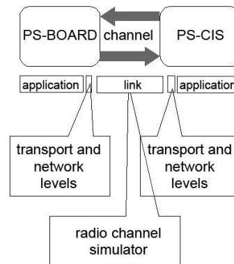
Fig. 2 - System architecture of PSS-TMS.
