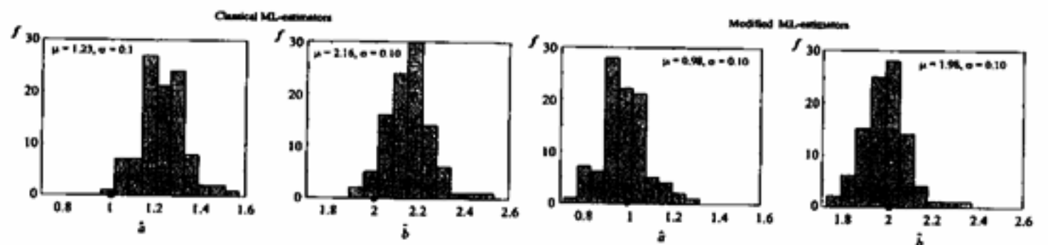
Figure 4: Histograms of the classical and proposed estimators of the BLM parameters for known distortion levels: f –empirical frequency, \mu – sample mean, \sigma –sample standard deviation; the circles denote the true parameter values.
