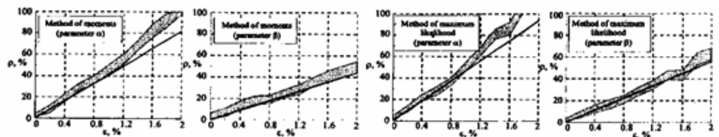
Figure 1: The biases of the classical MM- and ML-estimators of the BBM parameters, which ignore the misclassifications: gray tubes –experimental 95% confidence intervals; solid lines– approximation via the asymptotic expansions (7), (8); \rho –the relative bias, \varepsilon –the distortion level ( \varepsilon_0 = \varepsilon_1 ).
