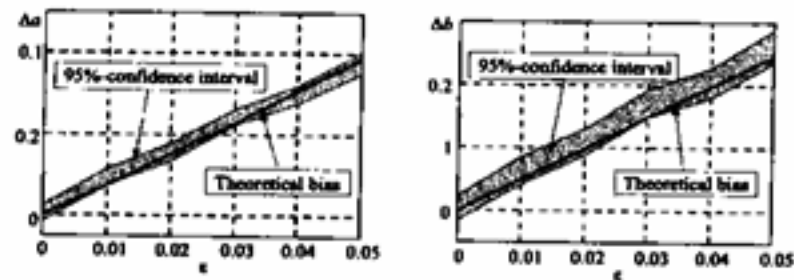
Figure 3: The biases of the classical ML-estimator of the BLM parameters, which ignores the misclassifications: gray tubes –experimental 95% confidence intervals; solid lines– approximation via the expansion (15); \Delta a, \Delta b –the relative bias, \varepsilon – the distortion level ( \varepsilon_0 = \varepsilon_1 ).
