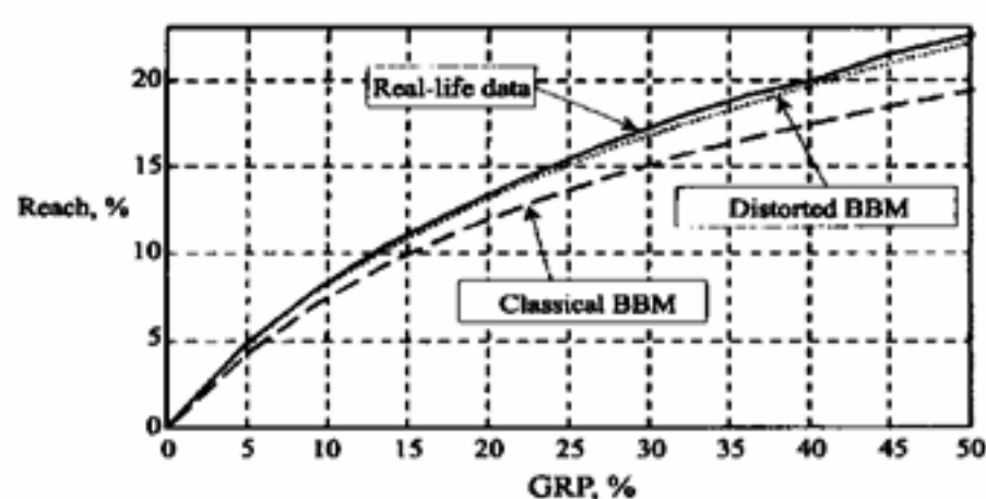
Figure 6: Comparison of the Reach–GRP curves based on the classical (BBM) and the proposed (DBBM) models against the curve obtained from the real data.
