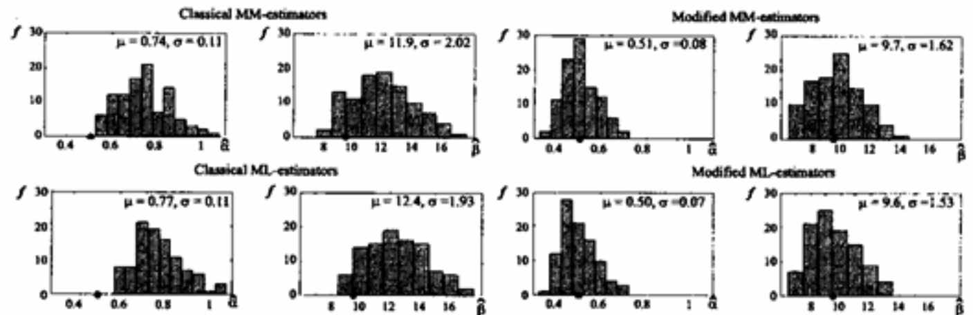
Figure 2: Histograms of the classical and proposed estimators of the BBM parameters for known distortion levels: f – empirical frequency, \mu – sample mean, \sigma – sample standard deviation; the circles denote the true parameter values.
