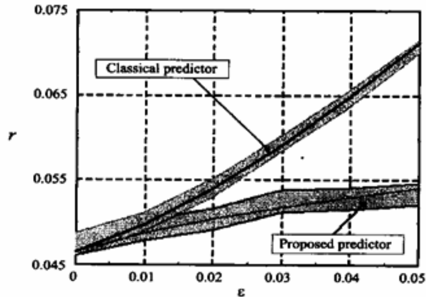
Figure 5: Comparison of the classical and proposed predictors: gray tubes – experimental 95% confidence intervals, solid lines – theoretical mean square errors of forecasting; r – mean square error, \varepsilon – distortion level ( \varepsilon_0 = \varepsilon_1 ).
