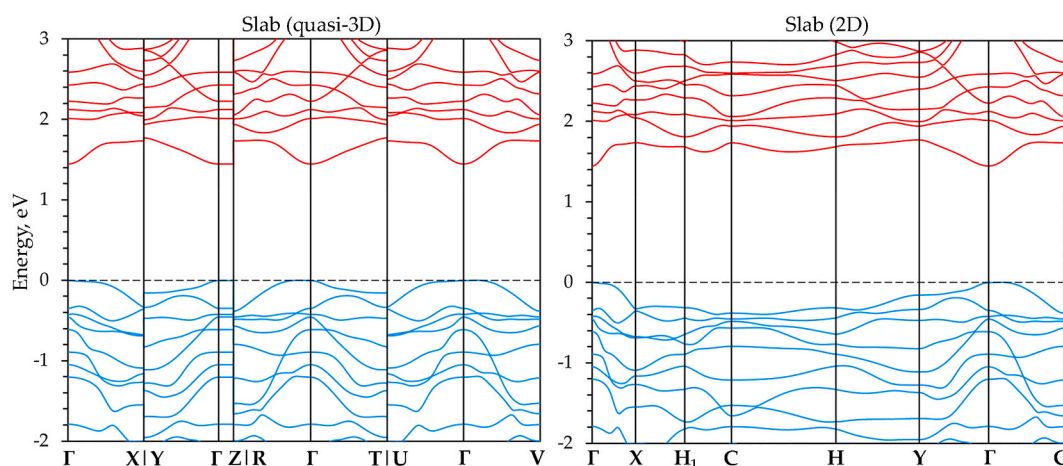
Fig. 4. Electronic band structure of \text{ReS}_2 monolayer, which unit cell is treated as quasi-3D (left panel) and as 2D (right panel). Zero is the upper valence band.
