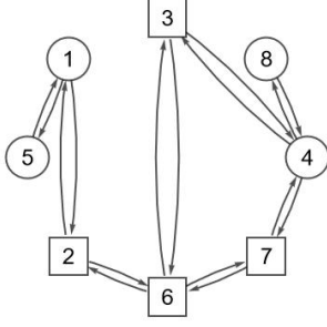
Fig. 1 – Graph G
