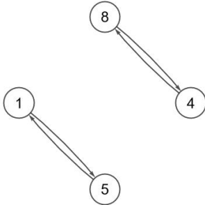
Fig. 2 – Graph G'
