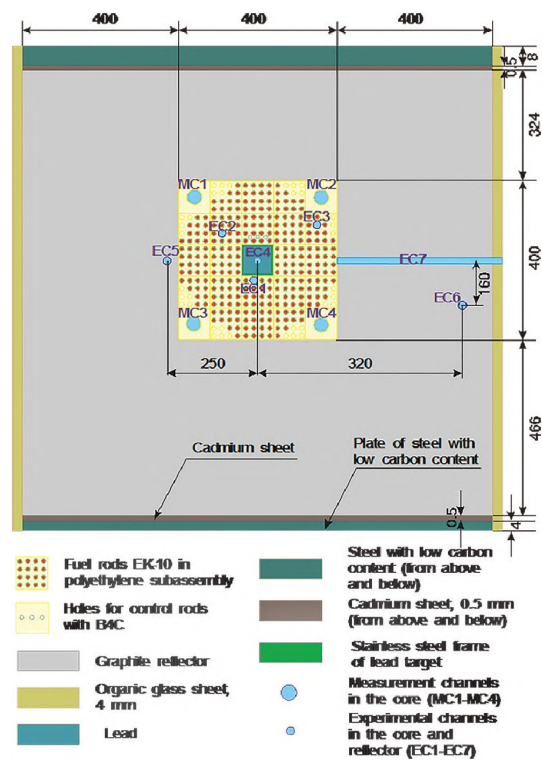
Fig. 1. The cross-section of YALINA-Thermal assembly
