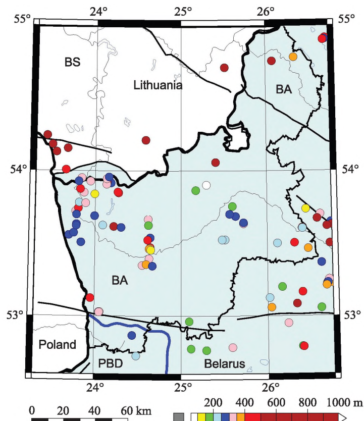
Fig. 3. Locations and depths of boreholes in the Grodno region with recorded thermograms. Here and in fig. 7–12 are given the following notations: BA – Belarusian Anticline; BS – Baltic Syncline; PBD – Podlasie – Brest Depression; PS – Polesian Saddle. The blue line shows the boundary of the Belarusian Anticline and the eastern part of the Podlasie – Brest Depression within Belarus. Black lines are the main faults
