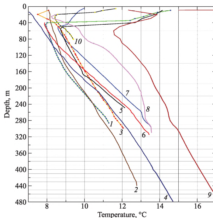
Fig. 4. Selected temperature logs of boreholes in the vicinity of Grodno: 1 – Grodno-10; 2 – Vorony-1; 3 – Grodno-8; 4 – Bershty-6; 5 – Grandichi-16; 6 – Tsydovichi-6; 7 – Grodno-1; 8 – Balesolnoye; 9 – Grandichi-15; 10 – Grodno-2a
