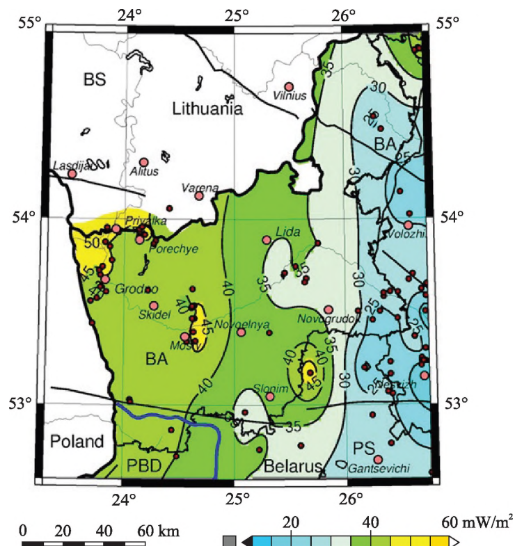
Fig. 11. Heat flow density map
