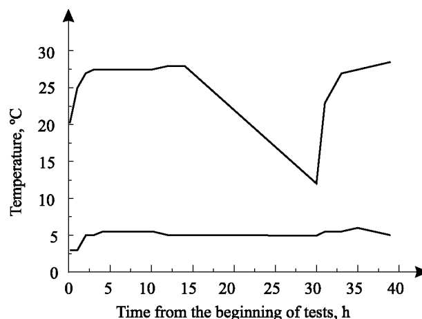
Fig. 3. Temperature variation diagrams at the inflow of the drilling mud into the drilling string (lower curve) and its outflow from the annular space (upper curve)
