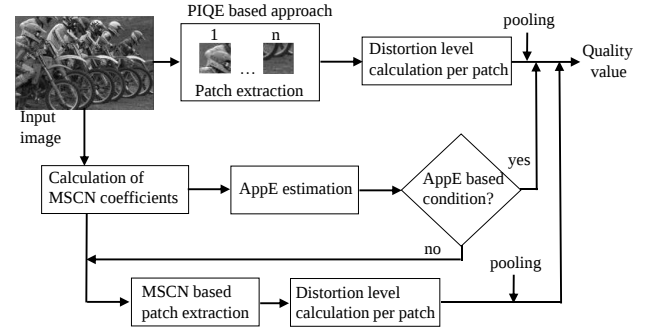
Fig. 1. AppE based perception framework for OU NR-IQA.
