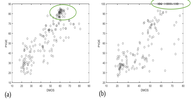
Fig. 2. High DMOS effects in PIQE versus DMOS comparison for: (a) jpeg and (b) ff impaired images.
