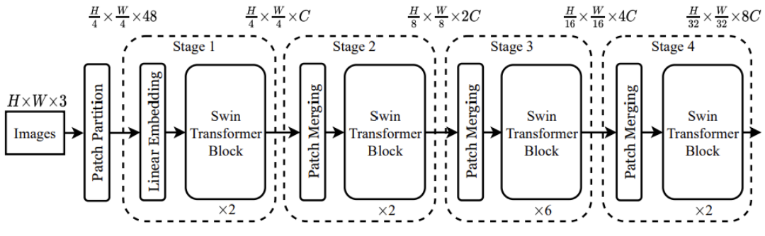
Fig. 4. The architecture of a Swin Transformer (Swin-T).
