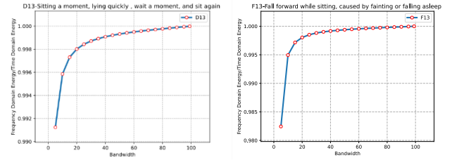
Fig 2. The curve graph of the energy ratio of 'Fall' and 'ADL'
