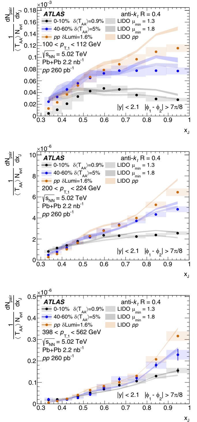
FIG. 12. The absolutely normalized x_J distributions for 100 < p_{T,1} < 112 GeV (top), 200 < p_{T,1} < 224 GeV (center), and 398 < p_{T,1} < 562 GeV (bottom) in pp collisions and for two centrality selections in Pb+Pb collisions. For Pb+Pb collisions, the measurements are compared with predictions from LIDO [42] for two values of the jet-medium coupling cutoff parameter, \mu_{\min} = 1.3 and \mu_{\min} = 1.8 , and the pp collision measurements are compared with the LIDO pp collision calculation.
