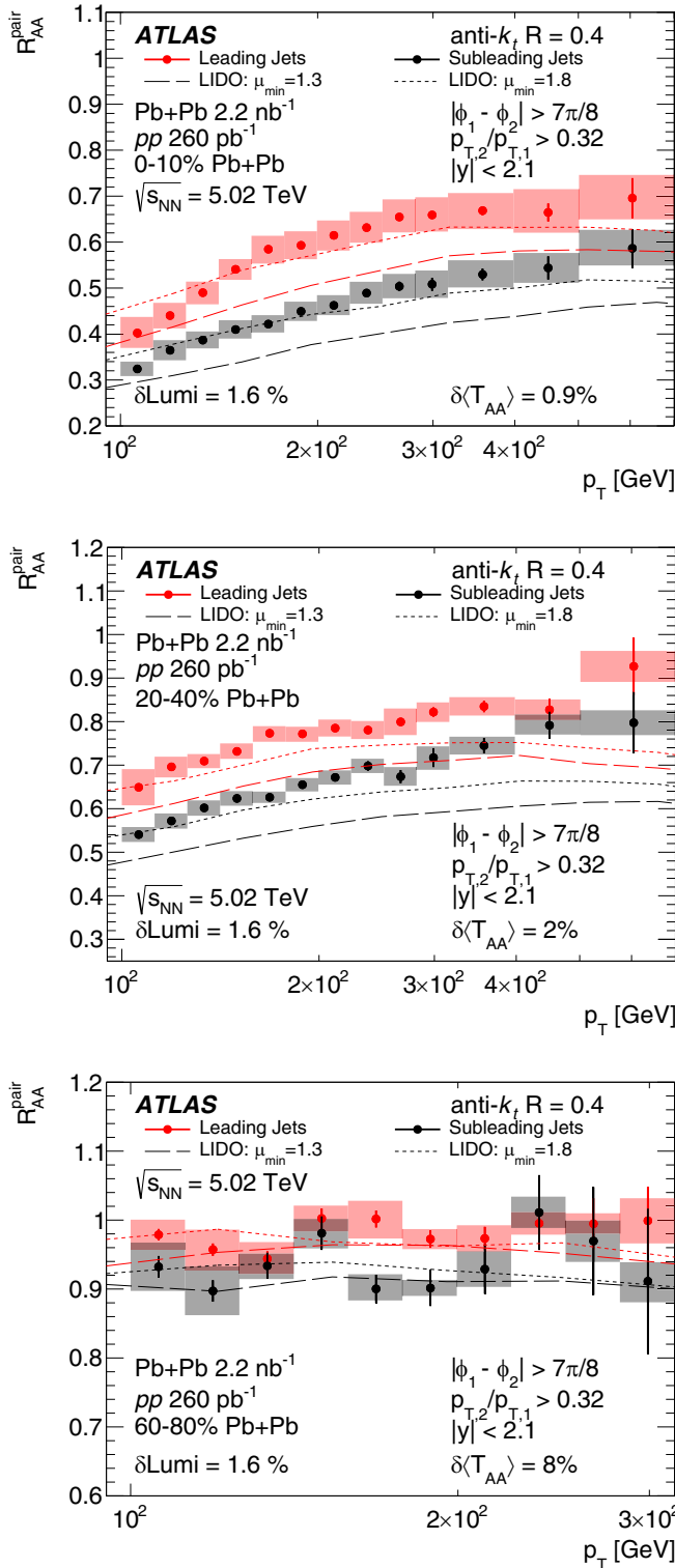
FIG. 13. The leading and subleading jet R_{AA}^{\text{pair}} distributions measured for a selection of centrality regions compared with predictions from LIDO [42]. Statistical uncertainties are shown as error bars (which are smaller than the markers in many cases) and systematic uncertainties are shown as boxes.
