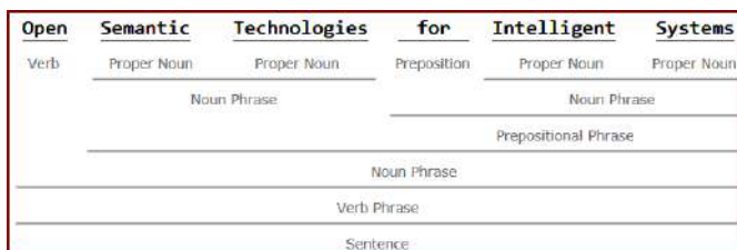
Figure 4. The result of executing the TextStructure function with the option "ConstituentTree".
