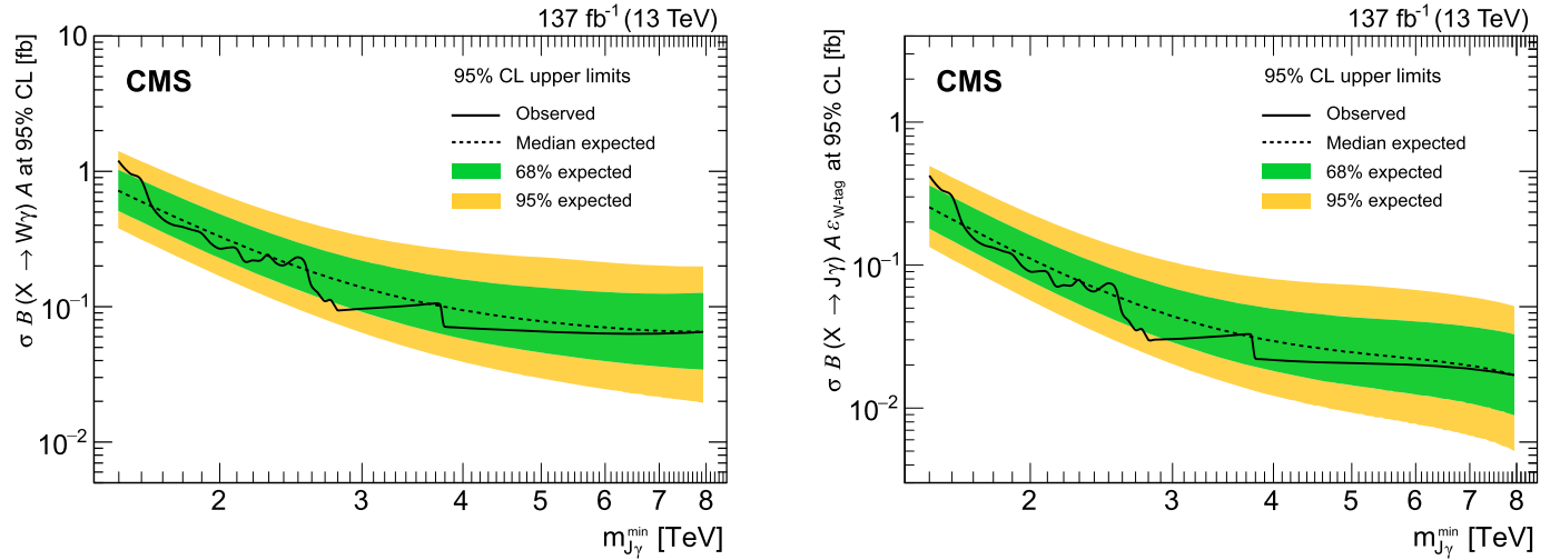
Fig. 7. Expected and observed 95% confidence level model-independent limits on \sigma\mathcal{B}(X \rightarrow W\gamma)\mathcal{A} (left) and \sigma\mathcal{B}(X \rightarrow J\gamma)\mathcal{A}\epsilon_{W\text{-tag}} (right), as a function of the minimum invariant mass requirement on the J\gamma system.
