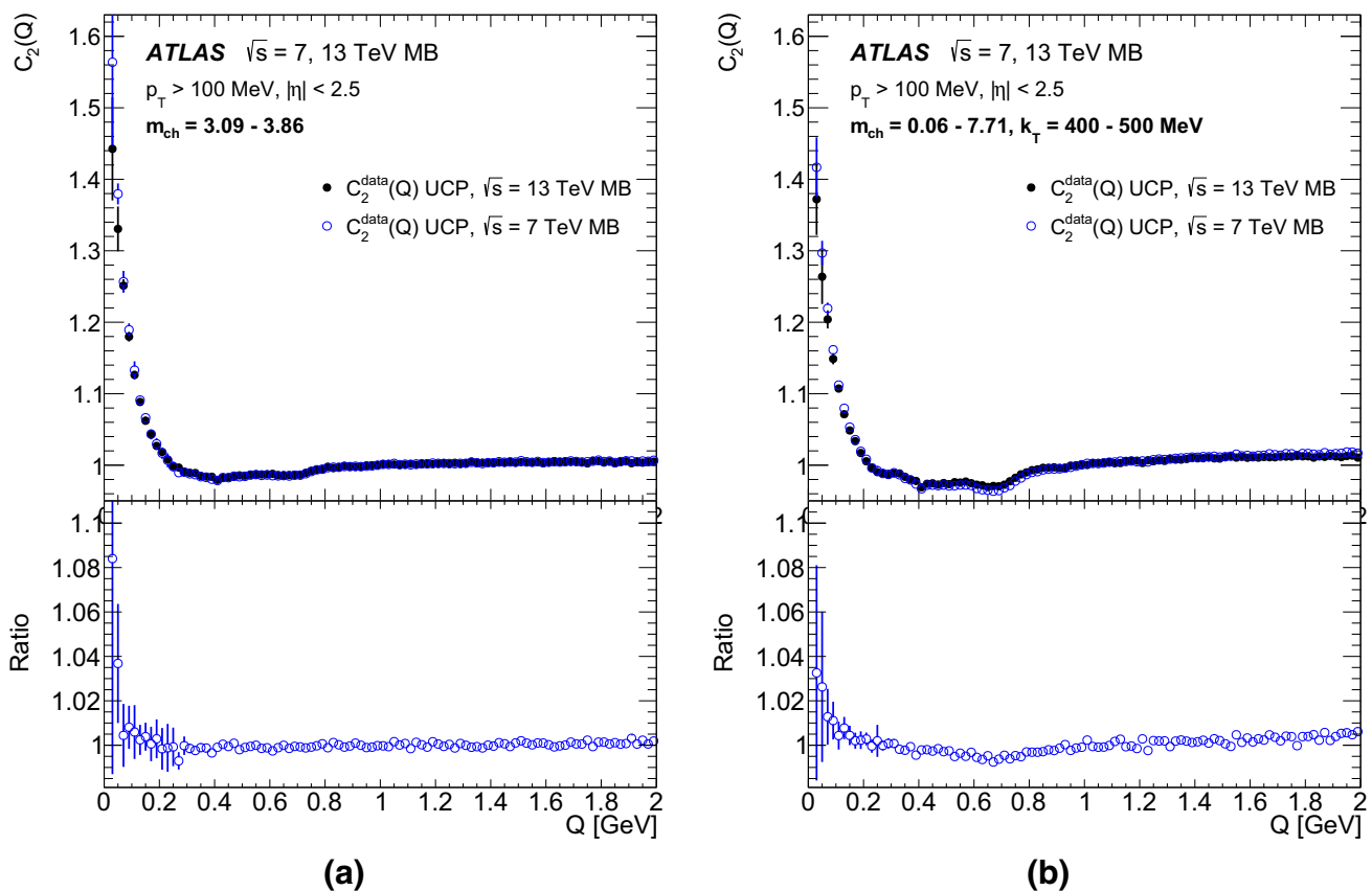
Fig. 5 Comparison of single-ratio two-particle correlation functions, using the unlike-charge particle (UCP) pair reference sample, for minimum-bias (MB) events, showing C_2^{\text{data}}(Q) (top panel) at 13 TeV (black circles) and 7 TeV (open blue circles), and the ratio of C_2^{13 \text{ TeV}}(Q) to C_2^{7 \text{ TeV}}(Q) (bottom panel). Comparison of C_2^{\text{data}}(Q) a for represen-
