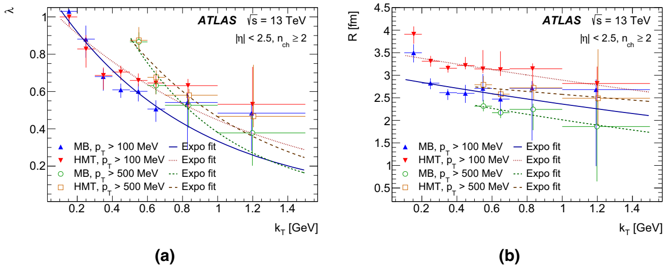
Fig. 6 The k_T dependence of a the correlation strength, \lambda(k_T) , and b the source radius, R(k_T) , obtained from the exponential fit to the R_2(Q) correlation functions for events with multiplicity n_{ch} \geq 2 and transfer momentum of tracks with p_T > 100 MeV and p_T > 500 MeV
