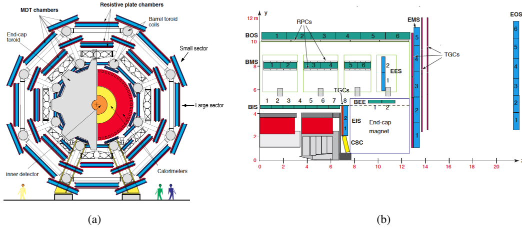
Figure 1. (a) View of the ATLAS MS barrel detectors in the transverse ( x, y ) plane. (b) View of the ATLAS MS layout in the (z, y) plane for a small azimuthal sector containing the barrel toroid coils. The green (blue) chambers are MDT chambers in the barrel (endcap) regions of the spectrometer. The TGCs, RPCs, and CSCs are shown in red, white, and yellow, respectively.
