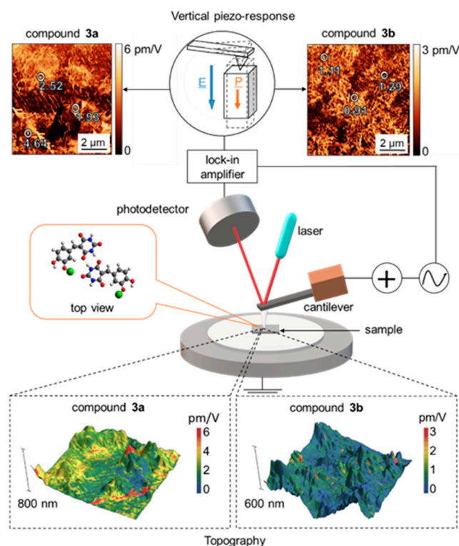
Figure 3. Surface topography and overlaid vertical piezoelectric responses of compounds 3a and 3b exposed to alternating voltage from PFM tip (probe spring constant is 10–12 N/m, working frequency is 20 kHz).
