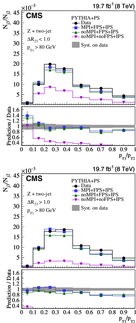
Fig. 8 Z + two-jet events at \sqrt{s} = 8 TeV compared to theoretical predictions from PYTHIA 8 without initial-state parton showers (IPS), final-state parton showers (FPS), and MPI: (upper) p_{T3}/p_{T2} for small-angle radiation ( \Delta R_{23} < 1.0 ), (lower) p_{T3}/p_{T2} for large-angle radiation ( \Delta R_{23} > 1.0 )
