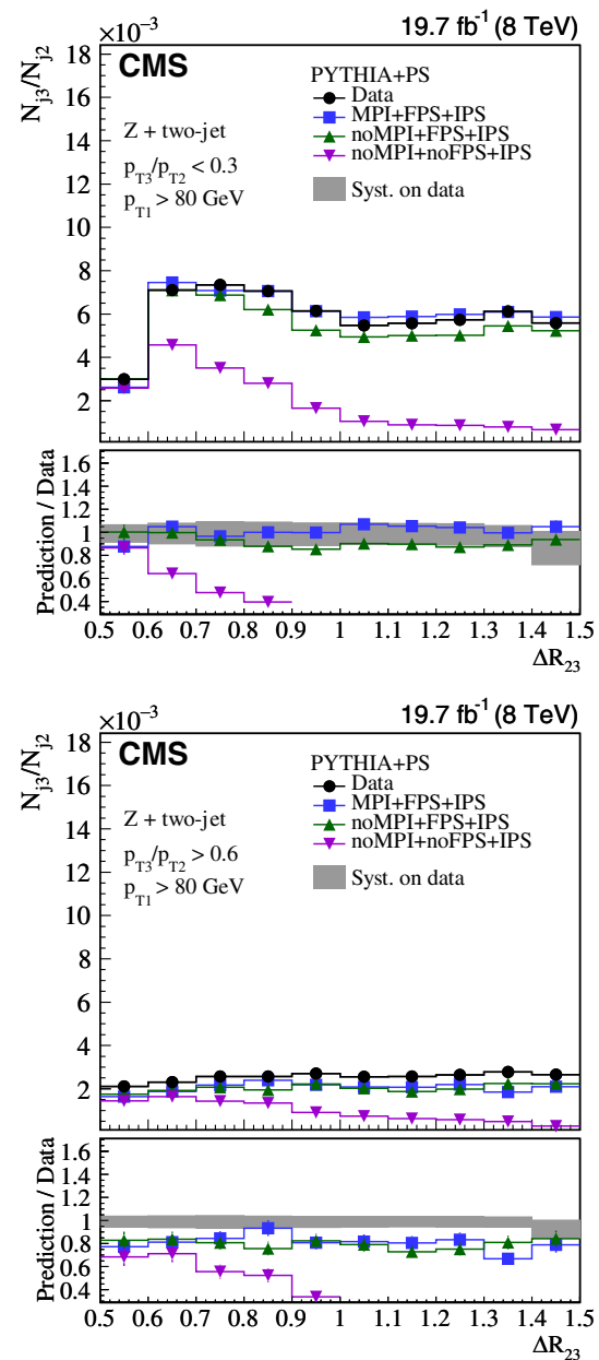
Fig. 9 Z + two-jet events at \sqrt{s} = 8 TeV and comparison to theoretical predictions from PYTHIA 8 without initial-state parton showers (IPS), final-state parton showers (FPS), and MPI: (upper) \Delta R_{23} for soft radiation ( p_{T3}/p_{T2} < 0.3 ), (lower) \Delta R_{23} for hard radiation ( p_{T3}/p_{T2} > 0.6 )
