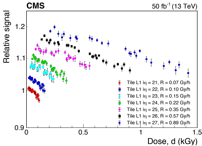
Figure 10. Relative signal for laser light versus accumulated dose for the SCSN-81 tiles in layer 1 with i\eta = 21 – 27 . The average dose rates are shown for each set of points. The vertical scale is logarithmic and subsequent sets are shifted up by a factor of 1.03 relative to the previous set for better visibility. Each set starts at the dose corresponding to integrated luminosity of 7 \text{ fb}^{-1} . Scaled statistical uncertainties are shown (see text).
