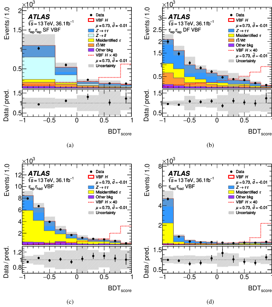
Fig. 2. Post-fit \text{BDT}_{\text{score}} distributions after the VBF event selection for the (a) \tau_{\text{lep}}\tau_{\text{lep}} SF, (b) \tau_{\text{lep}}\tau_{\text{lep}} DF, (c) \tau_{\text{lep}}\tau_{\text{had}} and (d) \tau_{\text{had}}\tau_{\text{had}} analysis channels. The ratios of the data to the prediction are shown in the lower panels. The observed VBF signal ( \mu = 0.73 , \bar{d} = -0.01 ) is shown with the solid red line on the top of the histogram stack. “Other bkg” denotes all background contributions not listed explicitly in the legend. The dashed line shows the observed VBF signal scaled up by a factor of 40 and is not part of the histogram stack. The size of the combined statistical, experimental, and theoretical uncertainties in the background is indicated by the hatched bands.
