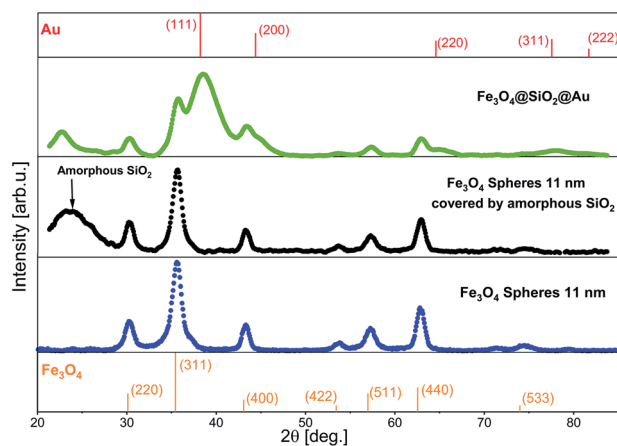
Fig. 5 XRD patterns of \text{Fe}_3\text{O}_4 , \text{Fe}_3\text{O}_4@SiO_2 and \text{Fe}_3\text{O}_4@SiO_2@Au NPs. On the top and on the bottom of the image standard references of Au and of \text{Fe}_3\text{O}_4 are added. 36,37
