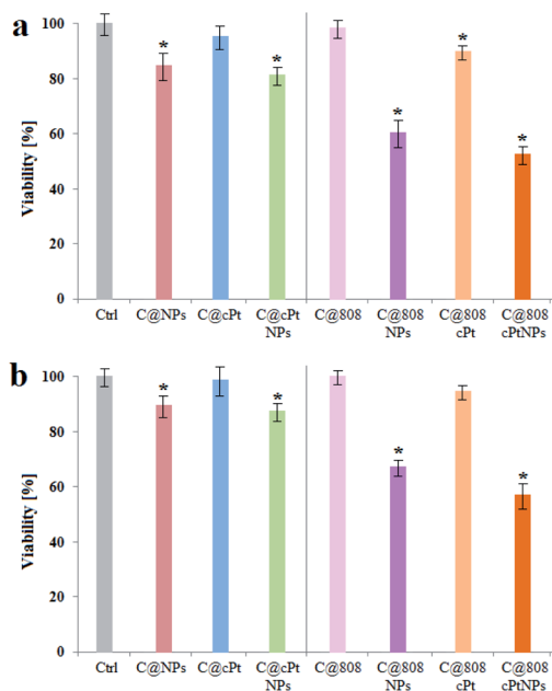
Fig. 12 Viability of colon cancer cells: SW480 (a); SW620 (b) after addition of cPt, \text{Fe}_3\text{O}_4@\text{SiO}_2@\text{Au} , functionalized \text{Fe}_3\text{O}_4@\text{SiO}_2@\text{Au} and laser irradiation in the presence of these three systems. Data was considered as significant when * p < 0.05 vs. control.
