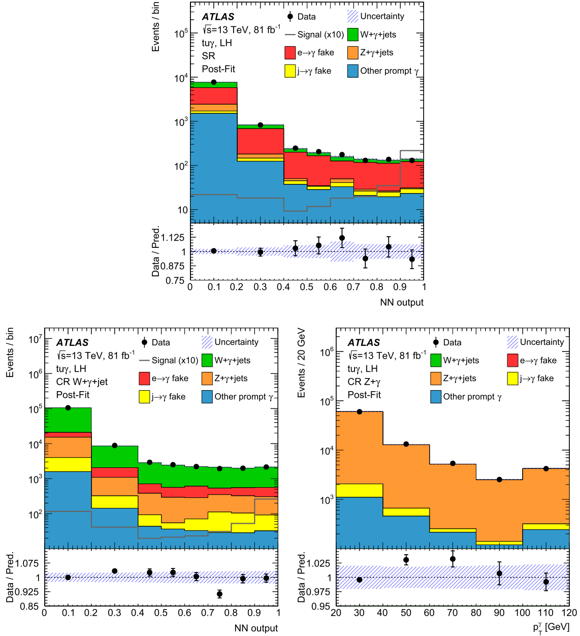
Fig. 2. Post-fit distributions of a background-only fit to the SR and the CRs of the NN output in the SR (top) and the W + \gamma + \text{jet} CR (bottom left) and of the p_T -distribution of the Z + \gamma CR (bottom right). The last bin of the distribution in the Z + \gamma CR contains the overflow. In addition, in the SR and in the W + \gamma + \text{jet} CR, the expected signal is overlaid for an effective coupling strength corresponding to the observed limit multiplied by a factor of ten. In the Z + \gamma CR, the expected signal is not shown, because it is negligible.
