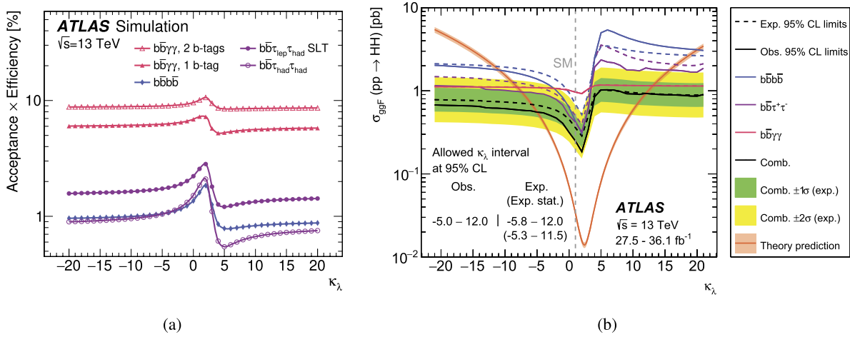
Fig. 4. (a) Signal acceptance times efficiency as a function of \kappa_\lambda for the b\bar{b}b\bar{b} , b\bar{b}\tau^+\tau^- and b\bar{b}\gamma\gamma analyses. The b\bar{b}b\bar{b} curve is the average of the 2015 and 2016 curves weighted by the integrated luminosities of the two datasets. (b) Upper limits at 95% CL on the cross-section of the ggF non-resonant SM HH production as a function of \kappa_\lambda . The observed (expected) limits are shown as solid (dashed) lines. In the b\bar{b}\gamma\gamma final state, the observed and expected limits coincide. The \pm 1\sigma and \pm 2\sigma bands are only shown for the combined expected limit. The theoretical prediction of the cross-section as a function of \kappa_\lambda is also shown. The effect of non-SM Higgs decay branching fractions due to \kappa_\lambda variations is not taken into account, which impacts the \kappa_\lambda intervals by no more than 7%.
