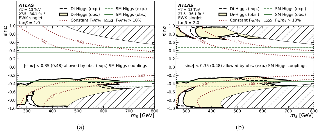
Fig. 6. Excluded regions for the EWK-singlet model for two values of the \tan \beta parameter: (a) \tan \beta = 1 and (b) \tan \beta = 2 . Indirect constraints from SM Higgs coupling measurements [74] are shown with horizontal lines. The dotted lines indicate the separation between regions where the resonance width is larger than 2% and 5% of the resonance mass. The hatch-marked area corresponds to regions that cannot be excluded because the width of the resonance exceeds 10% of the resonance mass, corresponding to the maximum of the experimental mass resolution among all analysed final states.
