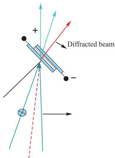
Fig. 3. Configuration of the experiment
