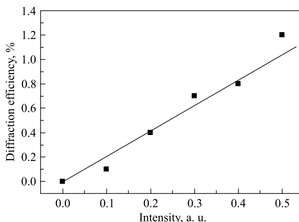
Fig. 4. Linear dependence of diffraction efficiency on the intensity of writing beams
