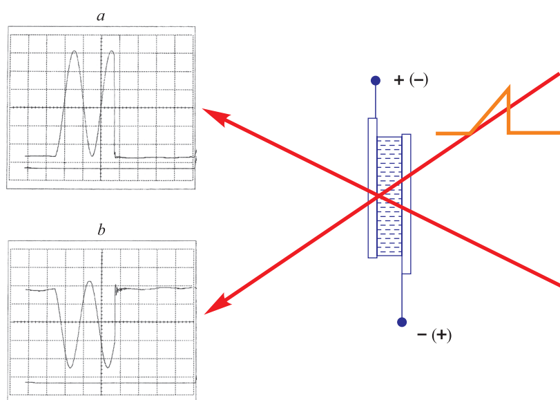
Fig. 7. Temporal behaviour of the writing beam in the moving grating experiment
