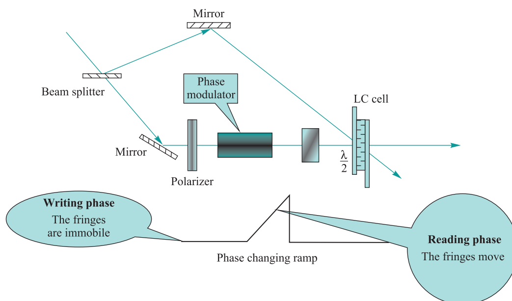
Fig. 6. Experimental set-up for moving grating measurement
