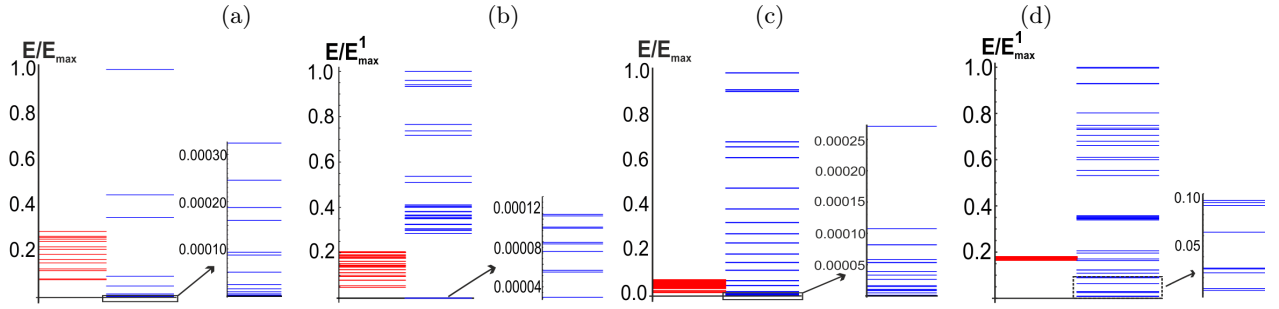
FIG. 3: Energy spectra for graphene quantum dots with topology S^1 \times S^1 (a, b) and S^2 (c, d) on low- (a, c) and high-energy scales (b, d). In each figure the left and right spectra correspond to the calculations in the folding-zone and pseudopotential-approximation approximations respectively. All spectra are normalized to the largest value of the right spectrum.
