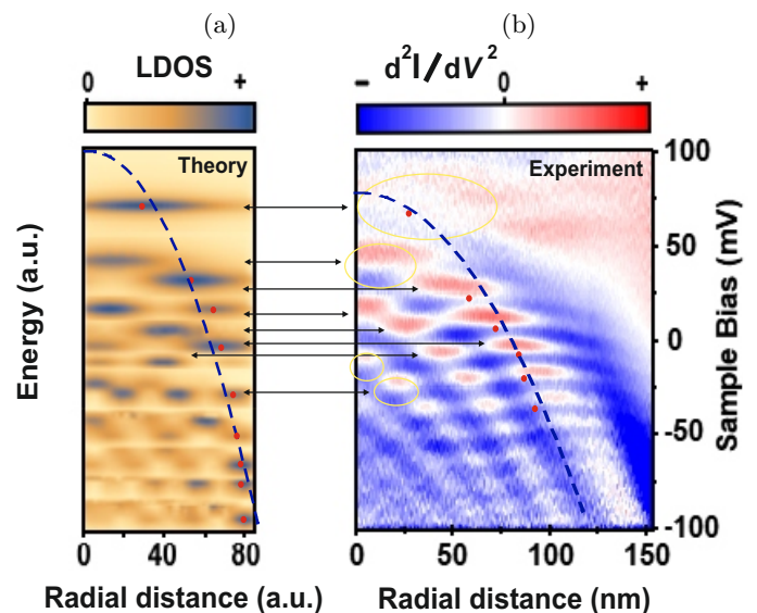
FIG. 9: Energy levels of spatially distributed states of a large graphene quantum dot. (a) Theoretically simulated LDOS in the bands of states confined by a pseudopotential for the continuous model of quantum dot with torus topology. (b) Second derivative \frac{d^2I}{dV^2} of a STM-current I measured as a function of the bias V and the radial distance from the center of a circular graphene p-n junction deposited on BN/SiO 2 . Lines with arrows indicate the theoretical bands, coinciding with experimental ones. Some resonances are encircled by yellow oval to improve perception. A fitting parabolic potential is indicated by a dashed line.
