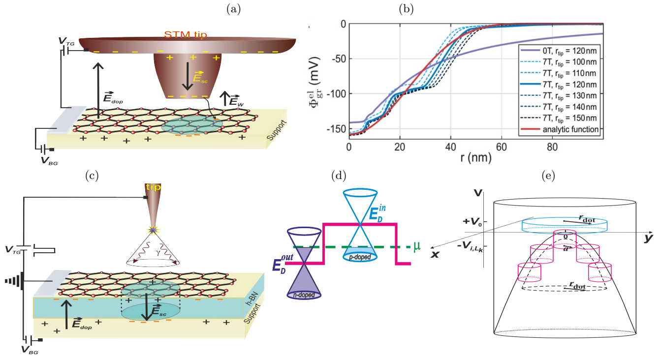
FIG. 1: A sketch of electrical fields creating circular graphene n-p and p-n junctions and the model potentials confining charge carriers in the junctions. (a) The n-p junction is induced by a STM double tip, which consists of a large-radius tip and a small-radius tip attached to the latter at the lowest point. Emerging at application of voltages V_{TG} and V_{BG} to the STM tip (top gate) and support (back gate) an electric field \vec{E}_{dop} dopes the bulk graphene with a positive charge. By polarizing the metallic thin tip one creates an electric field \vec{E}_{sc} , which screens the graphene region located under the tip from the action of \vec{E}_{dop} , that locally results in changing p-doping to n-doping. The level of n-doping also depends on the electric field \vec{E}_W = \Delta\vec{W}/e produced by the difference between work functions W_g and W_t of graphene and metal probe tip; (b) Cos-shape potential reconstructed on experimental data [4]; (c) The p-n junction is induced by a pulse of STM-tip voltage. The electromagnetic quanta \gamma polarize the h-BN region directly underneath the tip. The electric field \vec{E}_{sc} in this h-BN region functioning as a negatively charged local embedded gate positively dopes the graphene region underneath the tip. \vec{E}_{sc} screens the p-doped graphene region from an action of the electric field \vec{E}_{dop} which dopes bulk graphene with a negative charge; (d) Schematic of confining-potential measurements over two Dirac band touchings E_D^{in} and E_D^{out} inside and outside electrostatically confined graphene p-n junction respectively. The Dirac-touching offset produces a radial step potential V(r) . The chemical potential \mu is marked by a dashed line; (e) Model scattering potentials for the graphene quantum dot of radius r_{dot} : a long-wave approximation V_{i,R_k} \propto -\epsilon_{R_k}(q_i)\Theta(\lambda_i - R)\Theta(a - r) of pseudopotential (II.20) (red curves), R_k = |\vec{R} - \vec{r}| ; a parabolic potential (-\kappa r^2) with a large repulsive potential outside the graphene quantum dot (black curves); a cylindrical barrier potential V = +V_0\Theta(r_{dot} - R) \geq 0 , V_0 > 0 (blue curves). The +, - signs indicate the charge polarities in the tip and in graphene with support.
