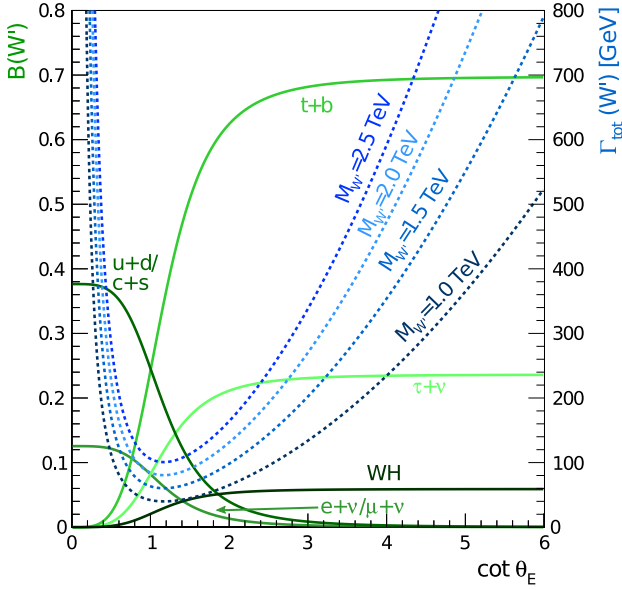
Fig. 1. Branching fractions (left-hand scale and solid lines) and total width (right-hand scale and dotted lines) for W' decays in the NUGIM, as calculated in Refs. [2, 11, 12]. For \cot\theta_E = 1 the values are the same as those in the SSM, rescaled to accommodate the WH decay channel.
