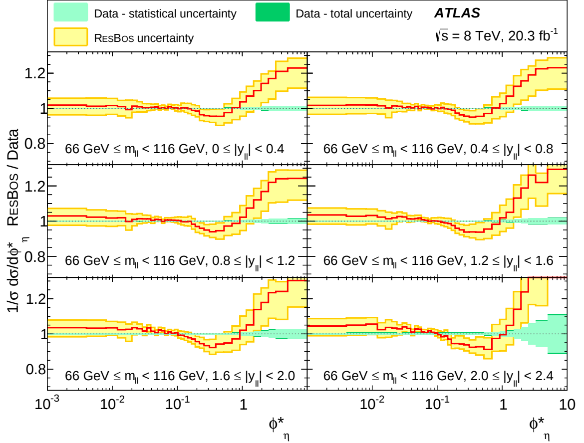
Figure 9: The ratio of (1/\sigma)d\sigma/d\phi_\eta^* as predicted by ResBos to the combined Born-level data, for the six |y_{\ell\ell}| regions at the Z-boson mass peak. The light-green band represents the statistical uncertainty on the data and the dark-green band represents the total uncertainty (statistical and systematic) on the data. The yellow band represents the uncertainty in the ResBos calculation arising from varying [53] the QCD scales, the non-perturbative parameter a_Z , and PDFs.
