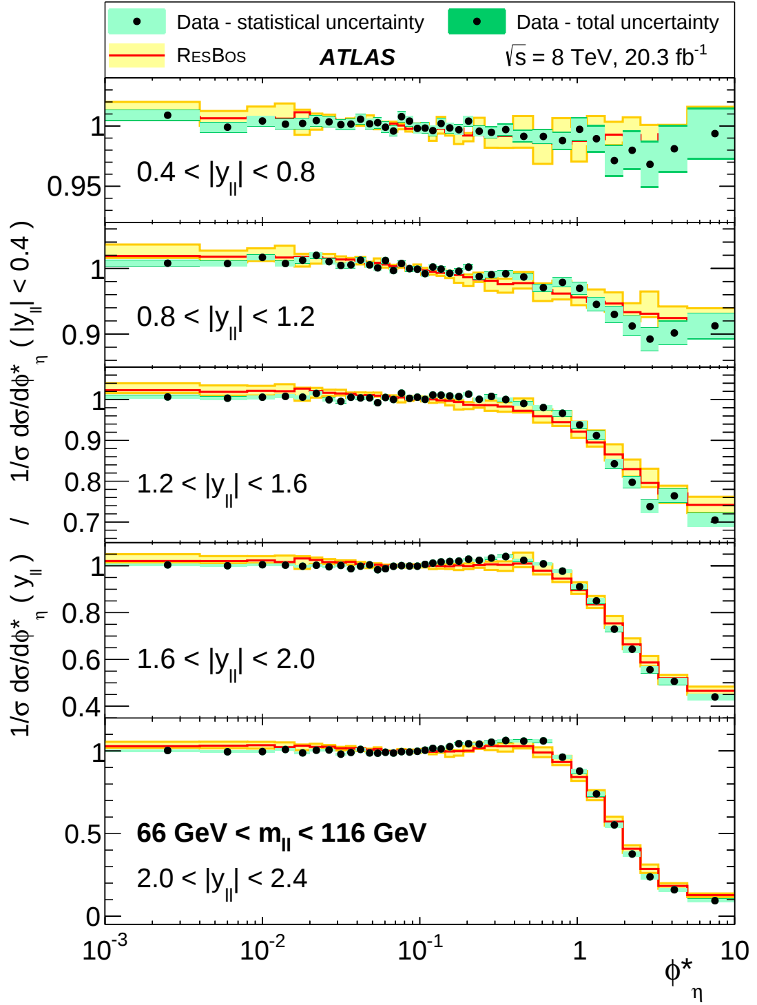
Figure 11: The distribution of (1/\sigma) d\sigma/d\phi_\eta^* at Born level in each region of |y_{\ell\ell}| , shown as a ratio to the central rapidity region ( |y_{\ell\ell}| < 0.4 ), for events at the Z-boson mass peak. The data, shown as points, are compared to the predictions of ResBos. The light-green band represents the statistical uncertainty on the data and the dark-green band represents the total uncertainty on the data (treating systematic uncertainties as uncorrelated between regions of |y_{\ell\ell}| ). The yellow band represents the uncertainty in the ResBos calculation arising from varying [53] the QCD scales, the non-perturbative parameter a_Z , and PDFs.
