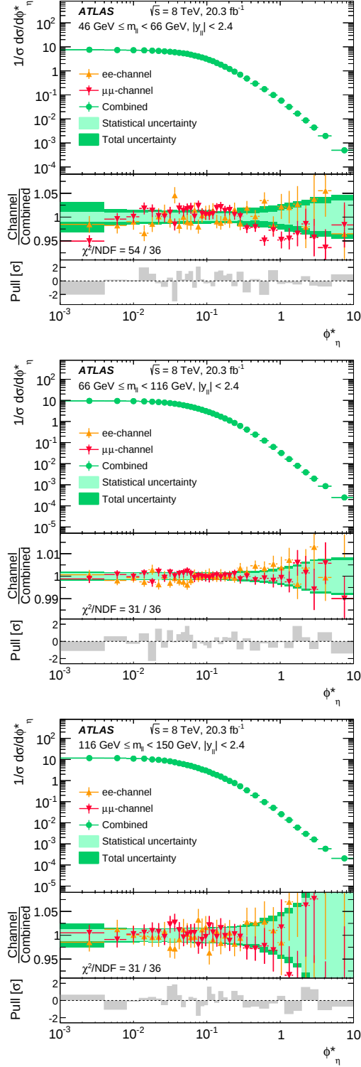
Figure 5: The Born-level distributions of (1/\sigma)d\sigma/d\phi_\eta^* for the combination of the electron-pair and muon-pair channels, shown in three m_{\ell\ell} regions from 46 GeV to 150 GeV for |y_{\ell\ell}| < 2.4 . The central panel of each plot shows the ratios of the values from the individual channels to the combined values, where the error bars on the individual-channel measurements represent the total uncertainty uncorrelated between bins. The light-green band represents the data statistical uncertainty on the combined value and the dark-green band represents the total uncertainty (statistical and systematic). The \chi^2 per degree of freedom is given. The lower panel of each plot shows the pull, defined as the difference between the electron-pair and muon-pair values divided by the uncertainty on that difference.
