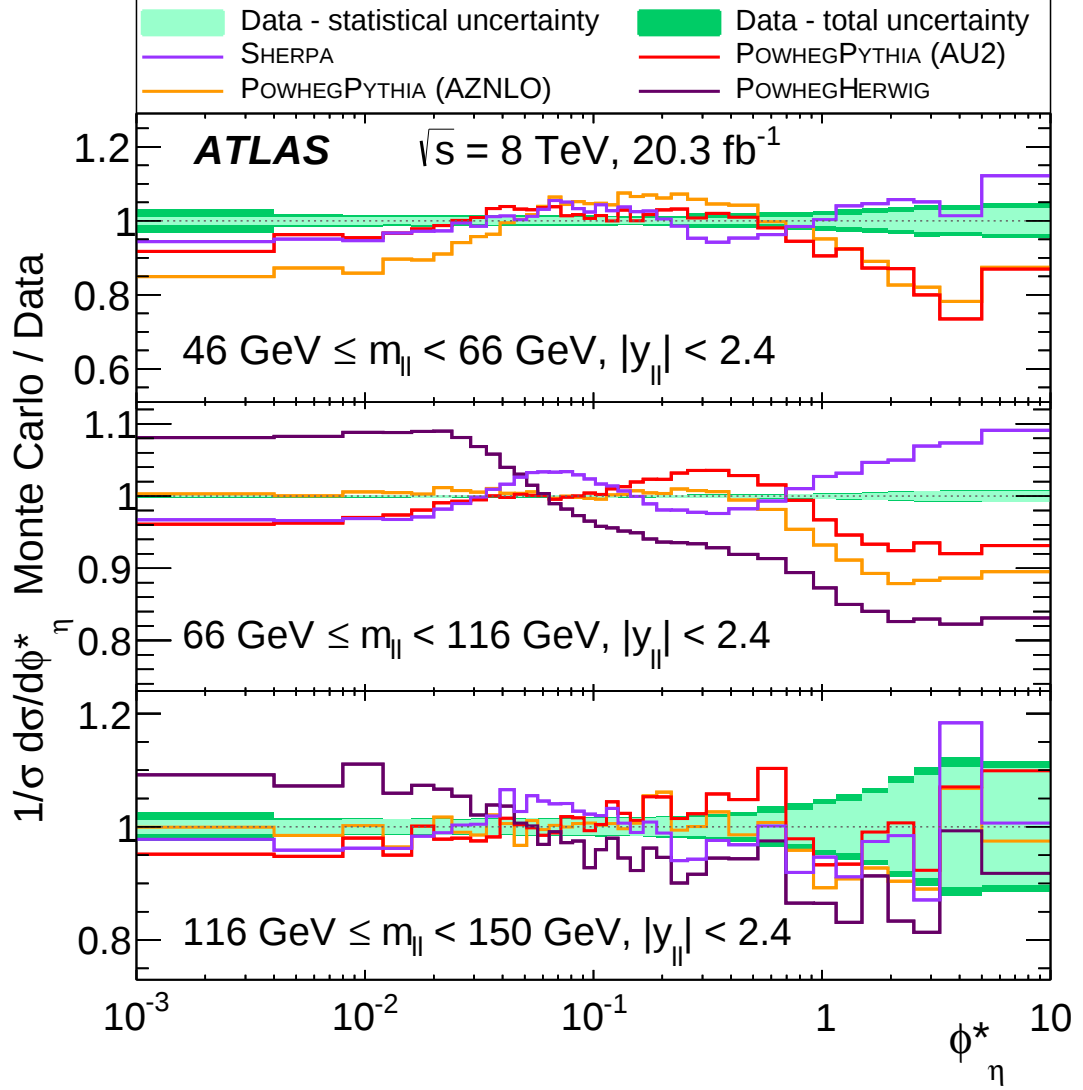
Figure 17: The ratio of (1/\sigma) d\sigma/d\phi_{\eta}^* as predicted by various MC generators to the combined Born-level data, in three different regions of m_{\ell\ell} for |y_{\ell\ell}| < 2.4 . The light-green band represents the statistical uncertainty on the data and the dark-green band represents the total uncertainty (statistical and systematic) on the data.
