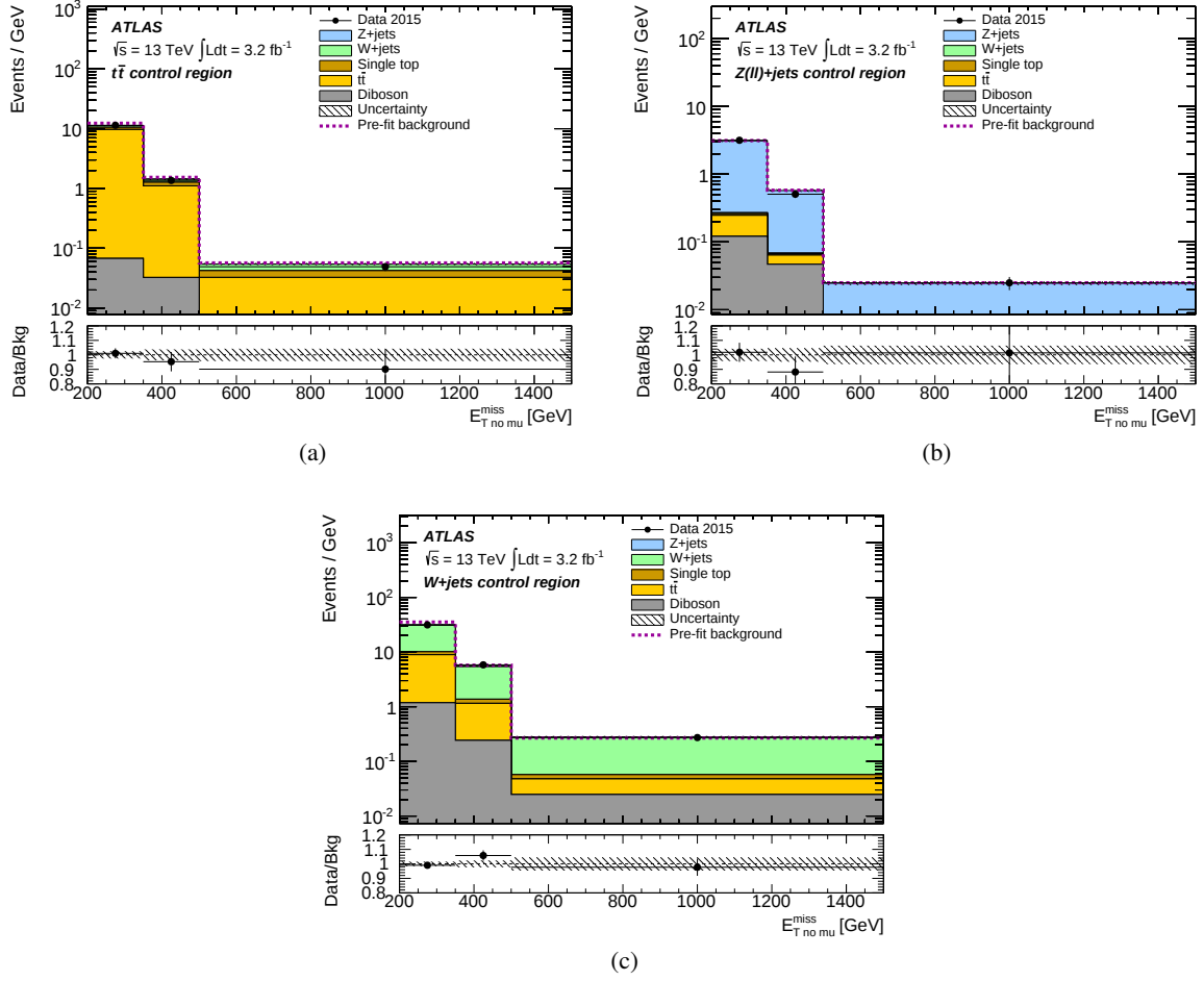
Figure 3: The E_T^{\text{miss}} distribution of the events in the control regions after the profile-likelihood fit to the data under the background-only hypothesis. Pane (a) shows the t\bar{t} control region, pane (b) shows the Z+l+jets control region, and pane (c) shows the W+l+jets control region. The total background prediction before the fit is shown as a dashed line. The inset at the bottom of each plot shows the ratio of the data to the total post-fit background. The hatched bands represent the total uncertainty in the background.
