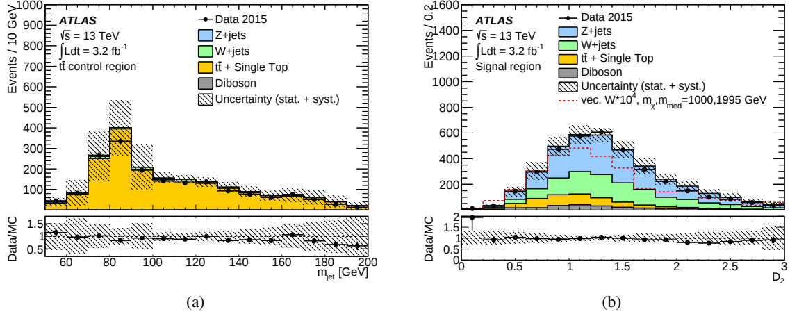
Figure 2: Pane (a) Distribution of m_{\text{jet}} in the data and for the predicted background in the top-quark control region. Pane (b) Distribution of jet substructure variable D_2 in the data and for the predicted background in events satisfying all signal region requirements other than those on D_2 . Also shown is the distribution for the simplified model with a vector-boson mediator, scaled by a factor of 10^4 for given values of m_\chi and m_{\text{med}} , the mediator mass.
