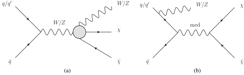
Figure 1: Pair production of WIMPs ( \chi\bar{\chi} ) in proton–proton collisions at the LHC in association with a vector boson ( V , meaning W or Z ) via two hypothetical processes: (a) production via an effective VV\chi\chi interaction or (b) via a simplified model which includes an s -channel mediator.
