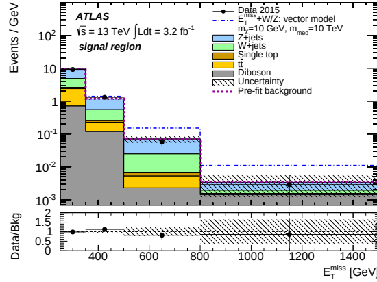
Figure 4: The E_T^{\text{miss}} distribution of the events in the signal region after the profile-likelihood fit to the data under the background-only hypothesis. The inset shows the ratio of the data to the total background. Also shown is the E_T^{\text{miss}} distribution for the simplified model with a vector-boson mediator, scaled by a factor of 10^4 for m_\chi = 10 GeV and m_{\text{med}} = 10 TeV. The total background before the fit is shown as a dashed line. The hatched bands represent the total uncertainty in the background.
