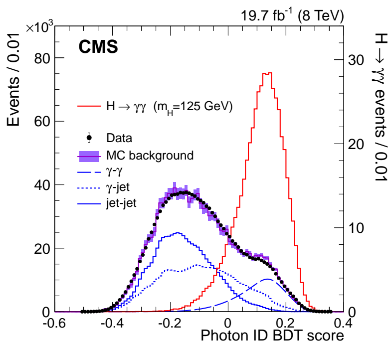
Figure 23: Photon identification BDT score of the lower-scoring photon of the diphoton pairs with invariant masses in the range 100 < m_{\gamma\gamma} < 180 GeV, for events passing the H \rightarrow \gamma\gamma preselection in the 8 TeV dataset (points with error bars), and for simulated background events (histogram with shaded error bands showing the statistical uncertainty). The solid line histogram on the right (righthand vertical axis) is for simulated Higgs boson signal events. Histograms are also shown for different components of the simulated background, in which there are either two, one, or zero prompt signal-like photons.
