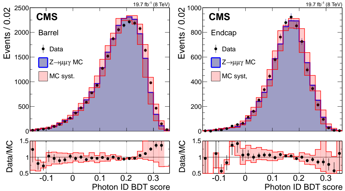
Figure 22: Identification BDT estimator for photons from Z \rightarrow \mu^+\mu^-\gamma with transverse momentum above 20 GeV. Data (points with error bars) are compared to Z \rightarrow \mu^+\mu^-\gamma events selected in Drell–Yan simulation (histograms). The shaded bands correspond to a shift of \pm 0.01 applied to the estimator value in simulation. The corresponding ratios of data to simulation are shown in the bottom panels.
