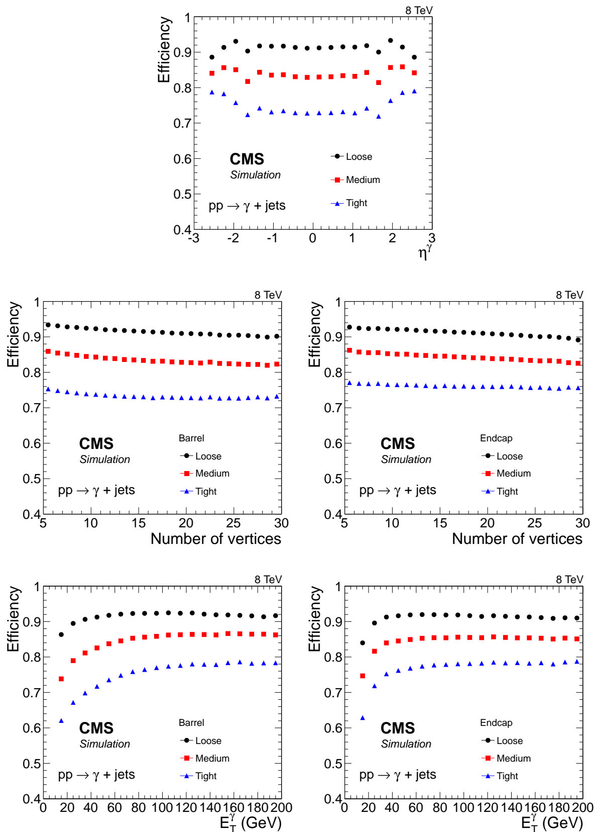
Figure 18: Efficiency of photon identification based on sequential requirements in simulated \gamma + \text{jet} events for three different working points, as a function of the (top) photon pseudorapidity, (middle) number of pileup vertices, and (bottom) photon transverse momentum. The efficiencies shown include the electron veto requirement.
