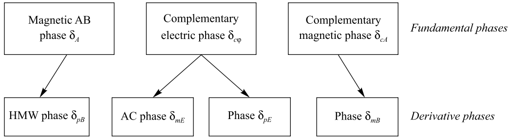
Relationship between velocity-dependent quantum phases for charged particles and for moving dipoles
