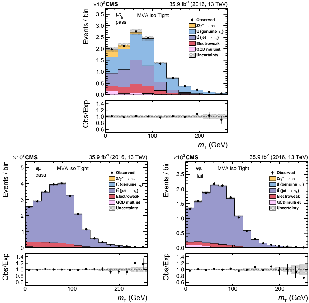
Figure 8. Fitted distributions for the signal (upper), e\mu passing (lower left), and the e\mu failing (lower right) categories, using the m_T for the \vec{p}_T^{\mu} and \vec{p}_T^{\text{miss}} vectors as observables for the tight WP of the MVA-based isolation with p_T^{\text{th}} between 30 and 40 GeV. The electroweak background includes contributions from W +jets (dominating), diboson, and single top quark events. Vertical bars correspond to the statistical uncertainties in the data points (68% frequentist confidence intervals), while the shaded bands reflect the quadratic sum of the statistical and systematic uncertainties after the fit.
