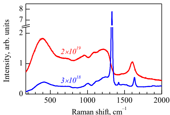
Figure 1. The Raman spectra of CVD DFs irradiated with fast neutrons with F = 3 \times 10^{18} and 2 \times 10^{19}\text{ cm}^{-2} . Measurements from the growth side, excitation wavelength is 532\text{ nm} .
