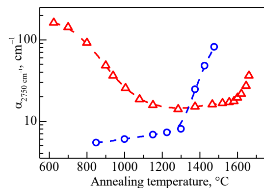
Figure 2. The effect of annealing in vacuum on the absorption coefficient at a frequency of 2750\text{ cm}^{-1} for unirradiated (circles) and irradiated with neutrons with a fluence of 2 \times 10^{19}\text{ cm}^{-2} (triangles) CVD DF.
