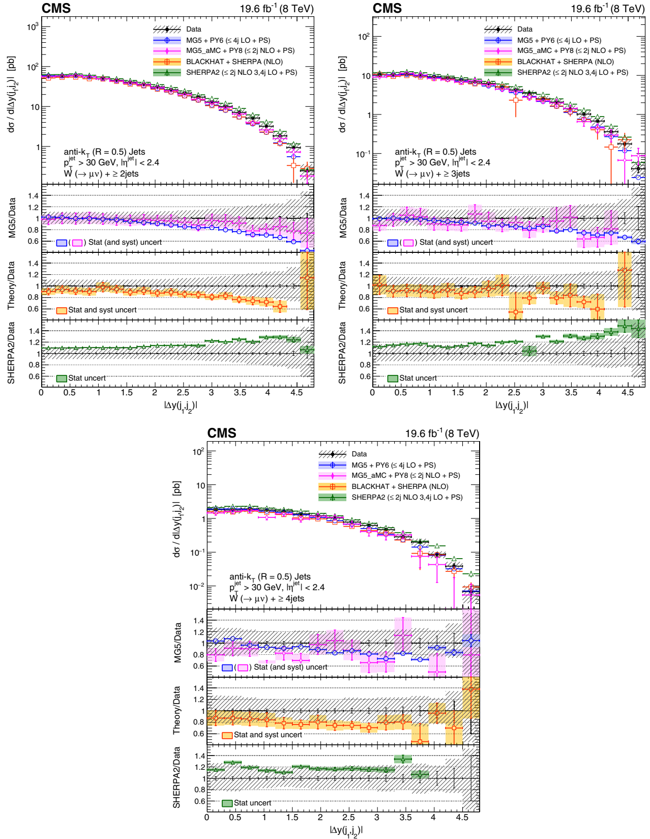
FIG. 9. Cross sections differential in \Delta y(j_1, j_2) for inclusive jet multiplicities 2–4, compared to the predictions of MADGRAPH, MADGRAPH5_aMC@NLO, SHERPA 2, and BLACKHAT+SHERPA (corrected for hadronization and multiple-parton interactions). Black circular markers with the gray hatched band represent the unfolded data measurements and their total uncertainties. Overlaid are the predictions together with their uncertainties. The lower plots show the ratio of each prediction to the unfolded data.
