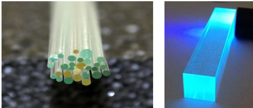
Figure 3. (left) Photograph of a bundle of 200 mm long fibers made of DSB:Ce with cross sections of \sim 1 mm. (right) First large volume sample made of DSB:Ce. The rectangular block with a volume of 23 \times 23 \times 120 mm 3 has been polished on all surfaces and is illuminated with a UV-lamp.
