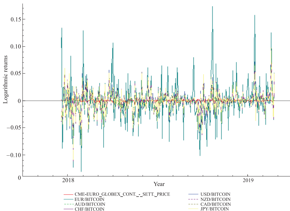
Fig. 1. Actual series of the logarithmic returns of the markets
