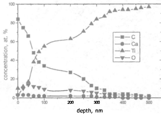
Fig. 6. Element distributions on a depth of the dental implant after irradiation (TEMP accelerator, E=300 keV; \tau=50 ns; n=5 pulses; j=120-150 A·cm 2 ).
