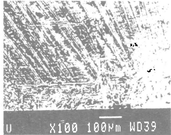
Fig.3. SEM micrograph of the dental surface HPPIB after irradiation (TEMP accelerator, E=300\text{ keV} ; \tau=50\text{ ns} ; n=5\text{ pulses} ; j=120\text{-}150\text{ A}\cdot\text{cm}^{-2} ).
