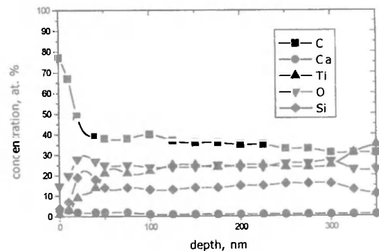
Fig.5. Element distributions on a depth of the dental implant after surface plastic straining (registration from the zone contented the conglomerate in Fig. 2).
