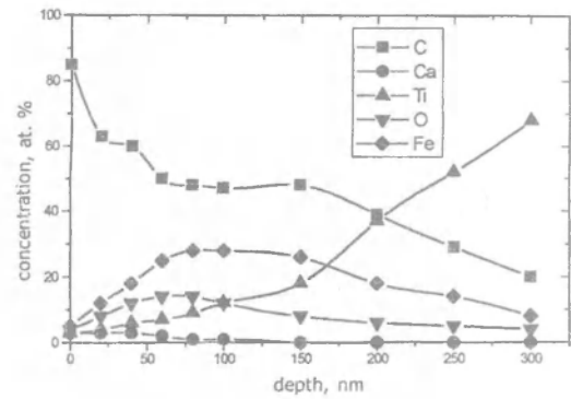
Fig.4. Element distributions on a depth of the dental implant after machining.
