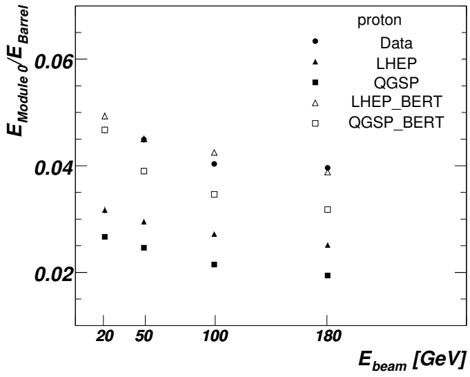
Figure 18: Ratio of energy depositions in the Module 0 to the ones in the Barrel Module for data and for various MC simulations as a function of the beam energy. Only statistical uncertainties are shown.
