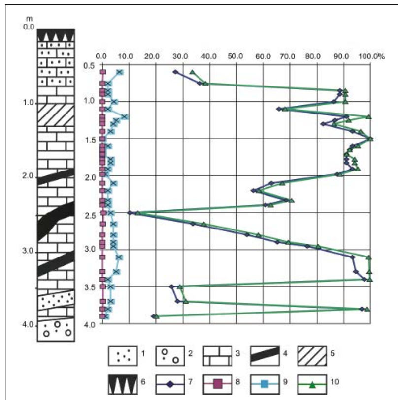
Fig. 3. Carbonate content in sediments the Dūkšta section.
