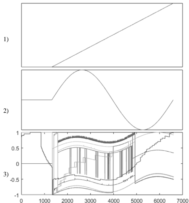
Fig. 4. – Modification of Dt_set_s1 data set: 1) Linearly increasing trend; 2) periodic component; 3) a modified multivariate signal.
