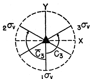
FIG. 2. The symmetry elements of C_{3v} .
