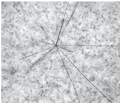
Fig. 1. Macrophotography of a star induced by a \mu -meson in it transversely exposed NTE.
