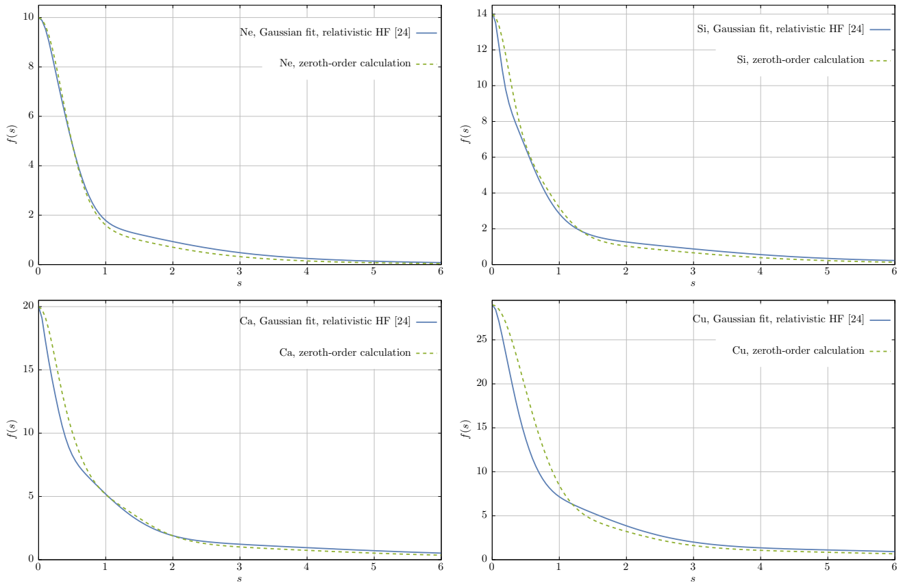
Figure 3. (color online) The dependence of the atomic scattering factors for Ne, Si, Ca and Cu atoms on the parameter s = \sin \theta / \lambda [\text{\AA}^{-1}] . The blue solid line is a gaussian fit taken from [24], the green dashed line is our analytical zeroth-order approximation.
