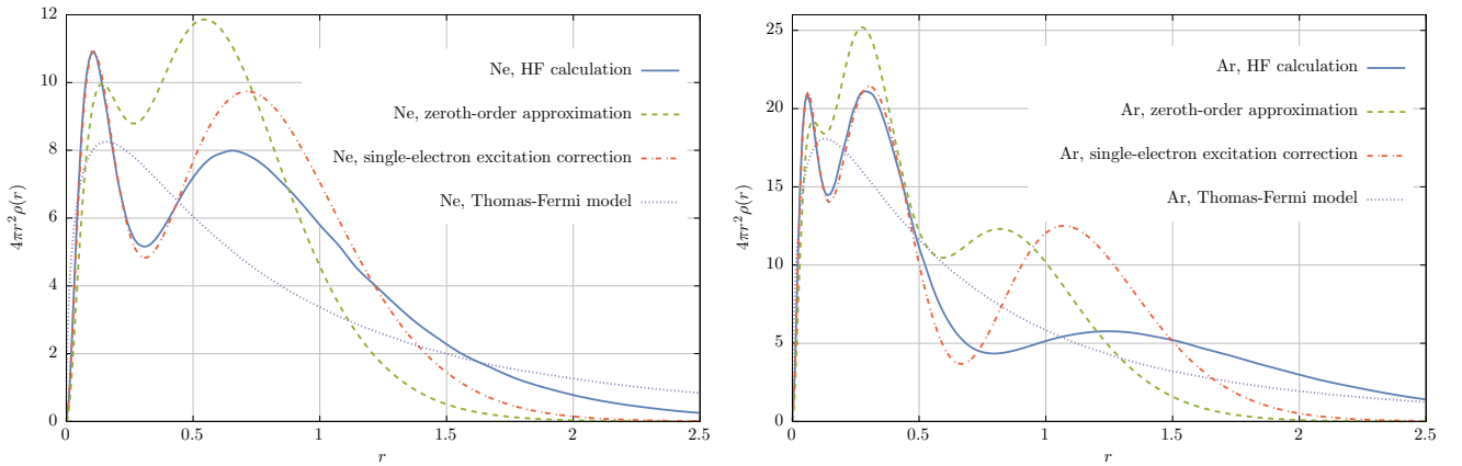
Figure 2. (color online) The dependence of the radial density Eq. (20) for Ne and Ar atoms on the radial coordinate r . The blue solid line is HF calculation [51, 62], the green dashed line is an analytical zeroth-order approximation, the red dashed-dotted line includes a single-electron excitation first-order correction and the purple dotted line is Thomas-Fermi model [48].
