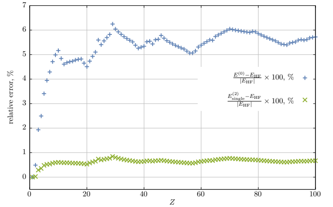
Figure 1. (color online) The relative error of the total atomic energy as a function of the nucleus' charge Z (the number of electrons is equal to Z ). The blue + -like crosses represent the relative error of the zeroth-order analytical energies and the green × -like crosses include the single-electron excitation correction. Both cases are compared to the corresponding HF results [50, 51].
