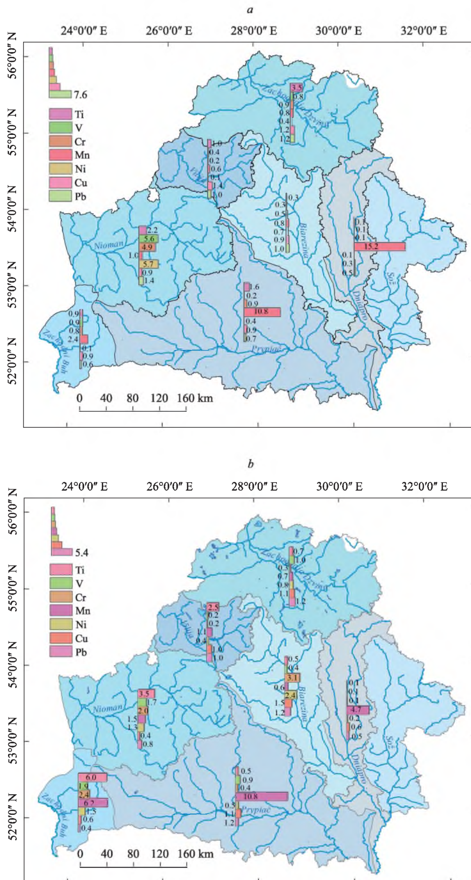
Fig. 3. Relative trace element abundances in emerged (a) and submersed with floating leaves (b) macrophytes of Belarusian lakes within principal river basins
