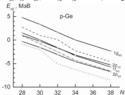
Fig. 1. Evolution of the proton single-particle energies of the neutron deficient Ge isotopes. Solid lines – calculation with DOP, dashed line – proton separation energy (with the opposite sign) from (N, Z+1) nuclei, dotted line – the same from (N, Z) nuclei, dashed-dotted line – the Fermi energy.
